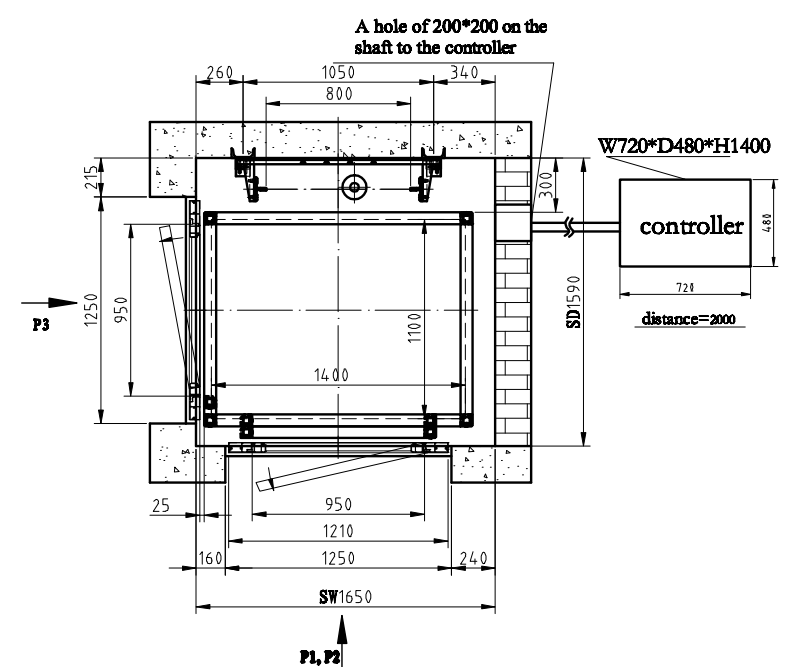
Shaft Plan 1: 30
