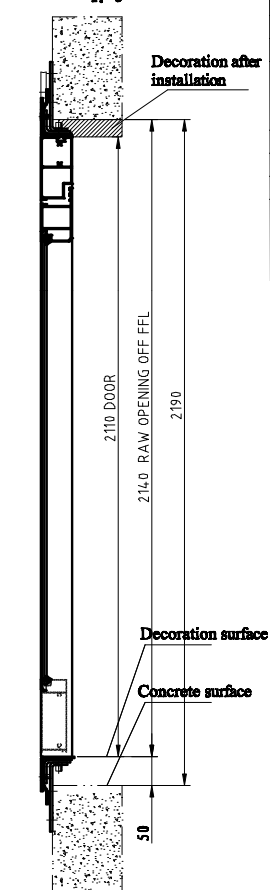
Sketch for landing door assembly 1: 8
