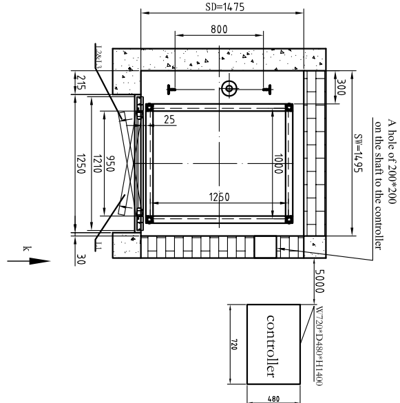
Shaft Plan
