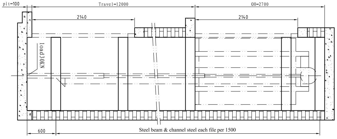
Shaft Section
